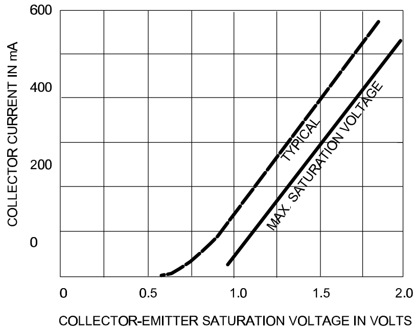
Figure 1-4, V_{ce}(\text{sat}) as a Function of Collector Current
